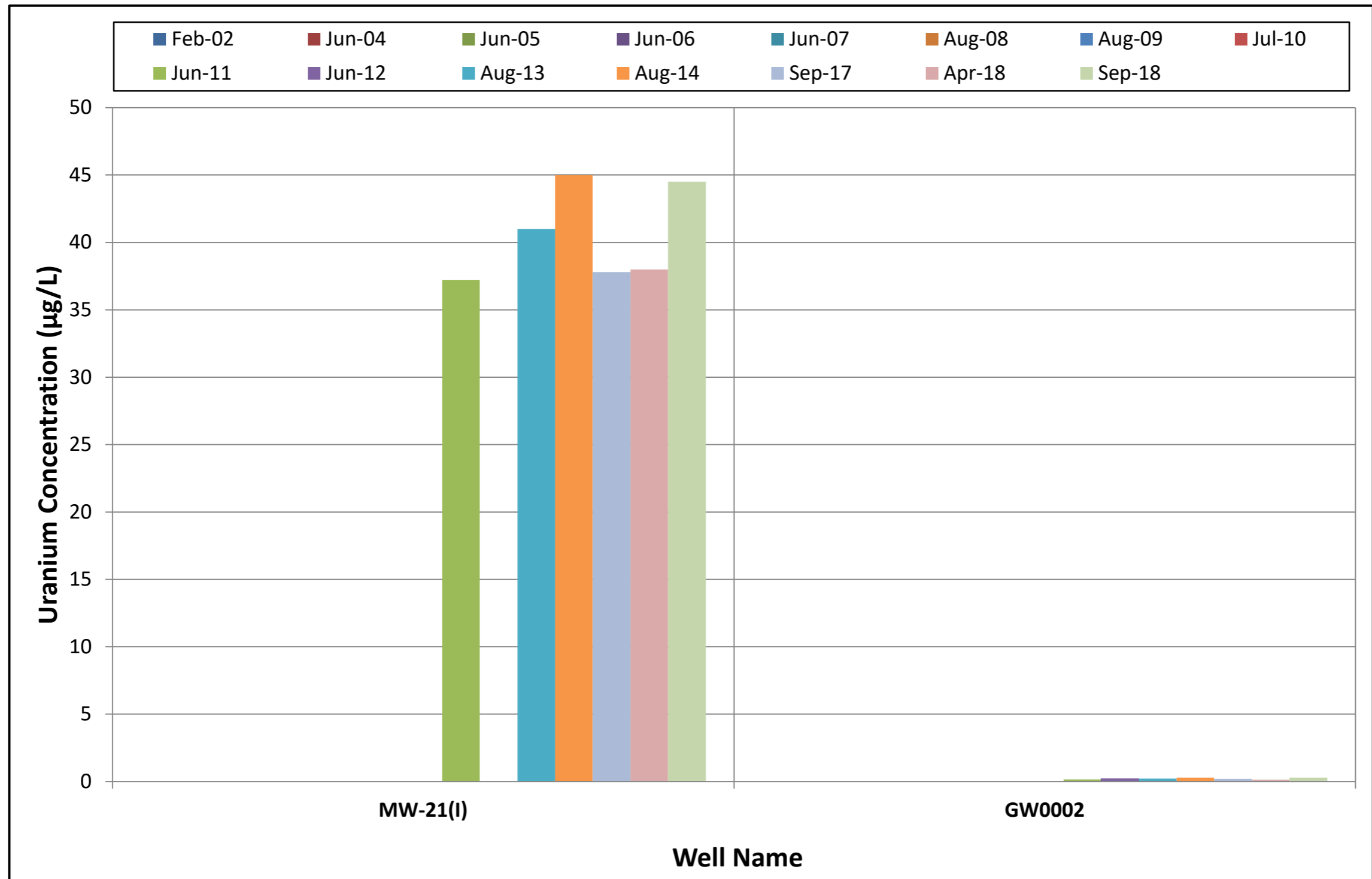
Figure 7: Uranium Concentrations in Filtered Groundwater
