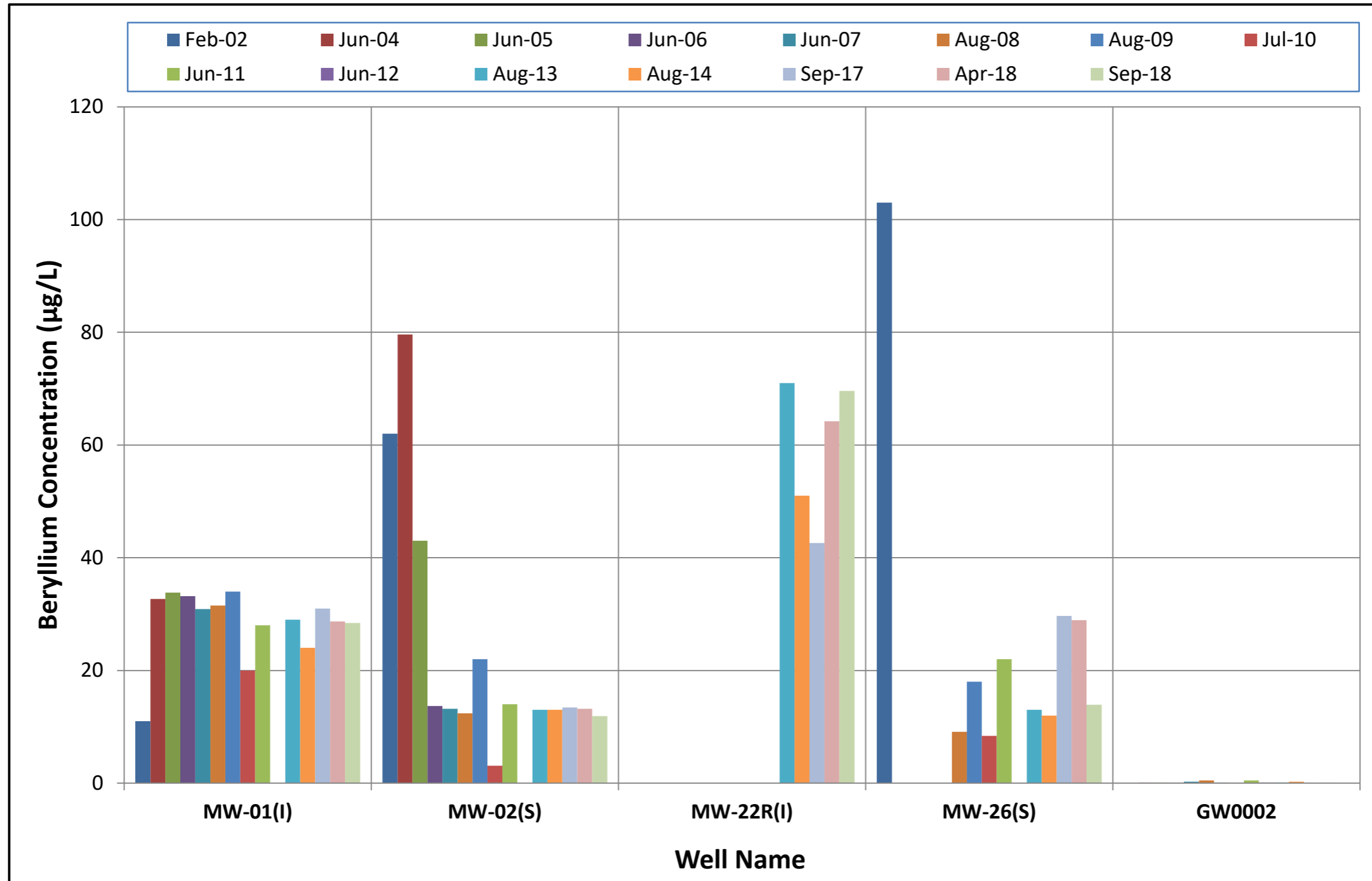
Figure 3: Beryllium Concentrations in Filtered Groundwater
