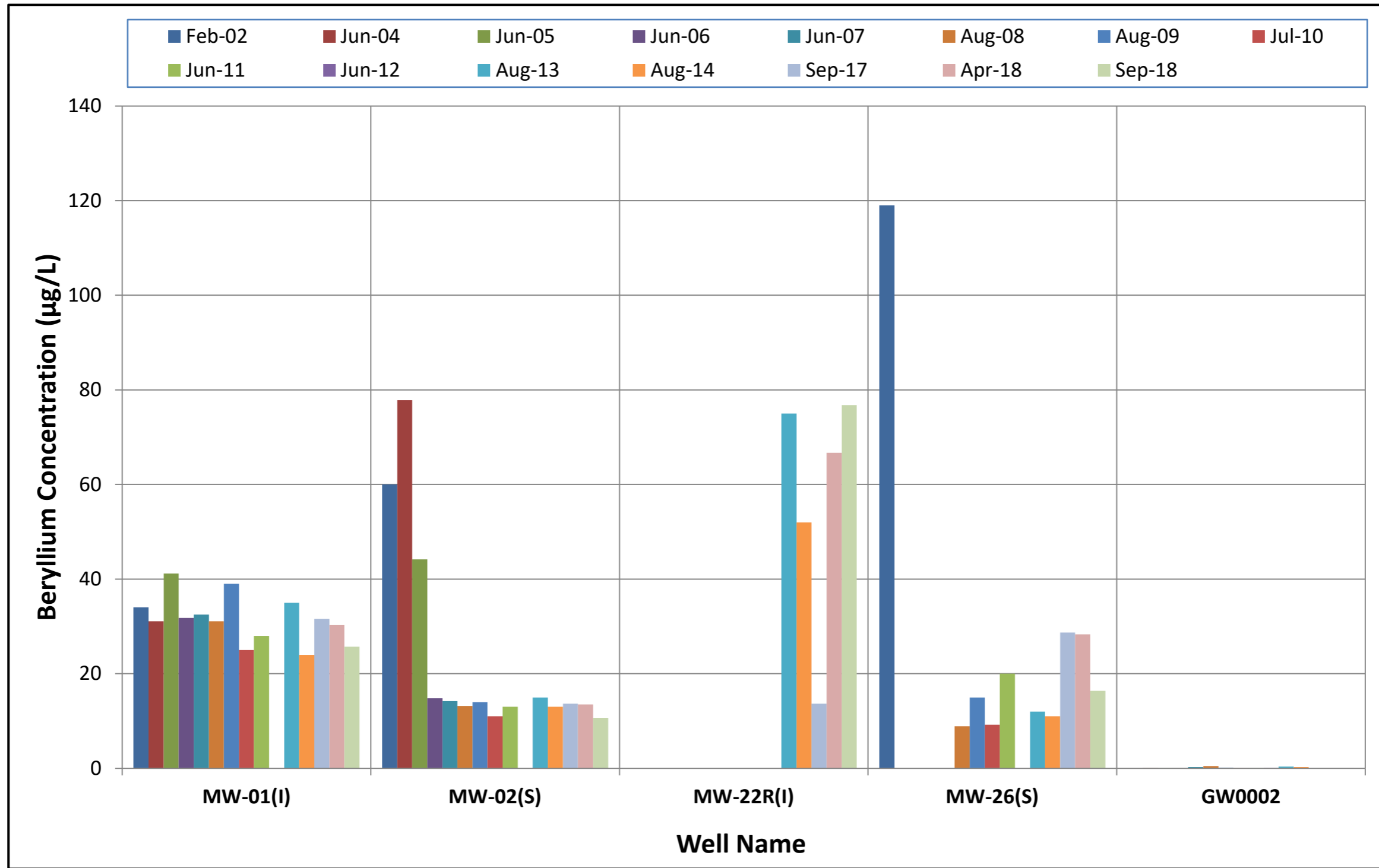
Figure 2: Beryllium Concentrations in Unfiltered Groundwater
