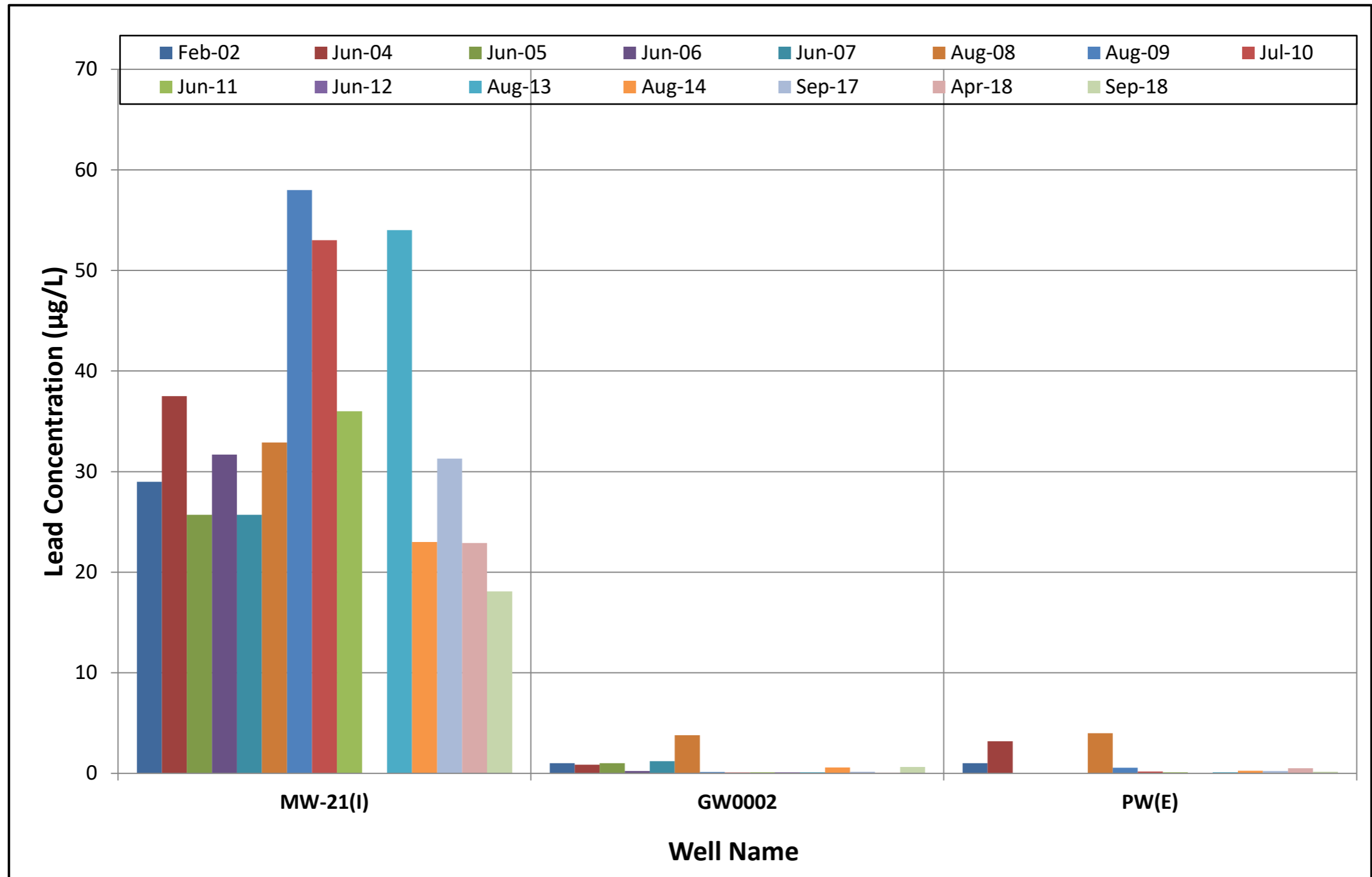
Figure 5: Lead Concentrations in Filtered Groundwater
