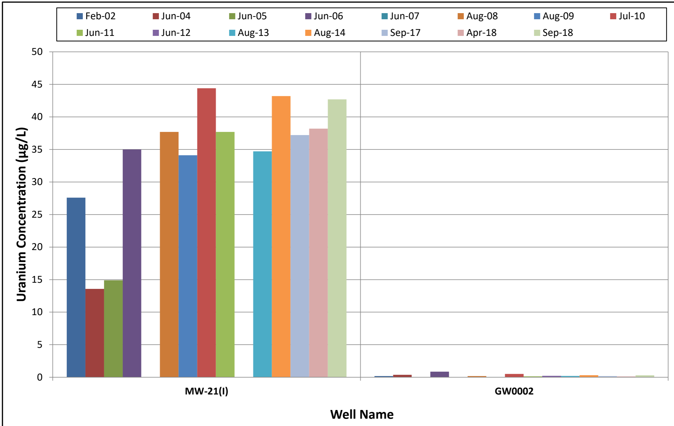
Figure 6: Uranium Concentrations in Unfiltered Groundwater
