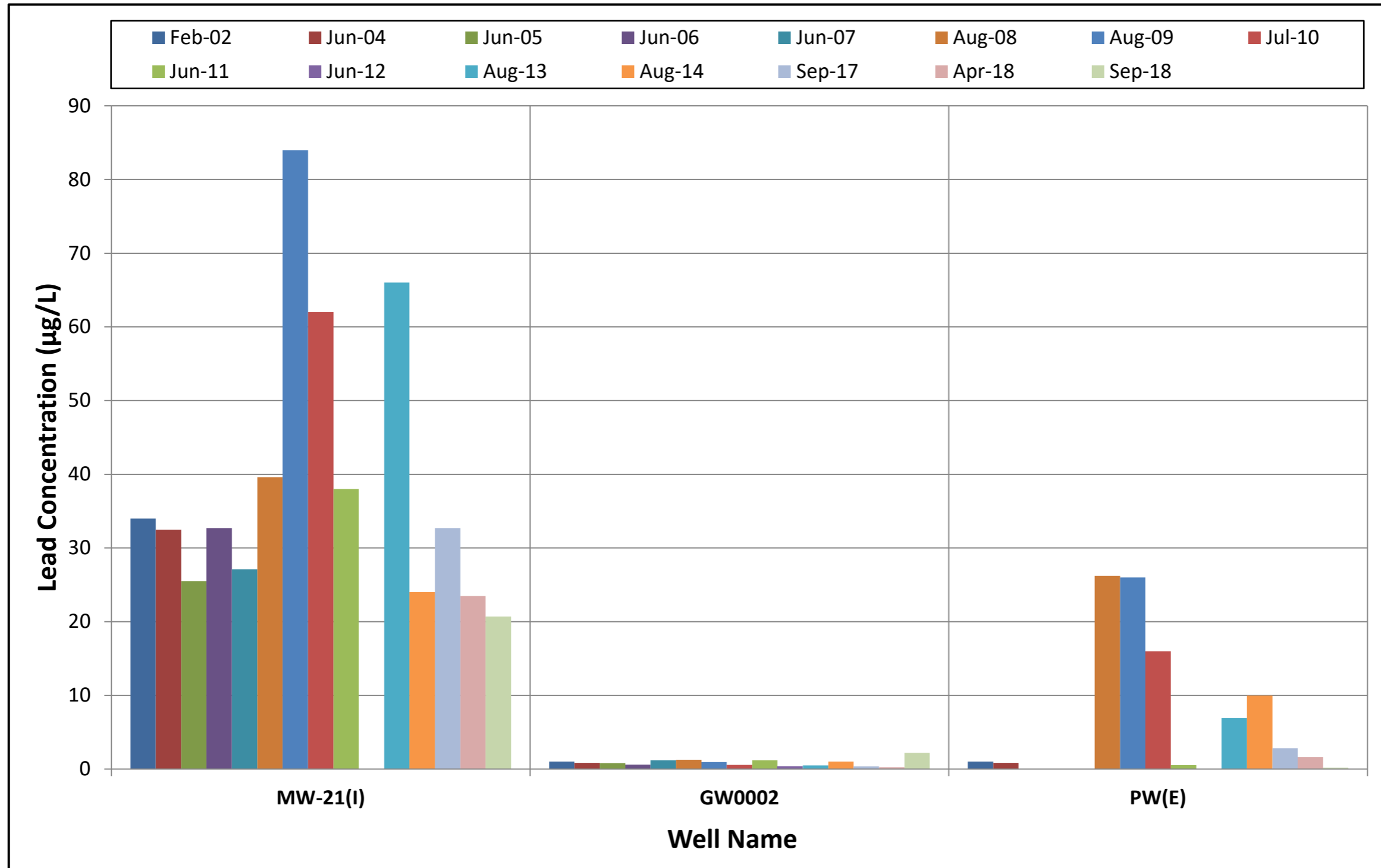
Figure 4: Lead Concentrations in Unfiltered Groundwater
