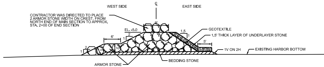
TYPICAL CROSS SECTION - END SECTION CONSTRUCTED 2021
